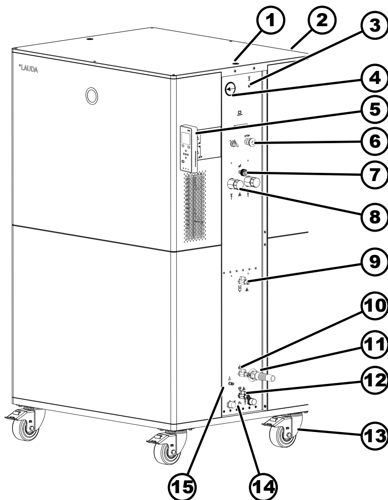
Fig. 7: Vue Integral IN 2040 PW
