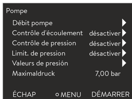
Fig. 36: Menu Pompe Integral IN XT
